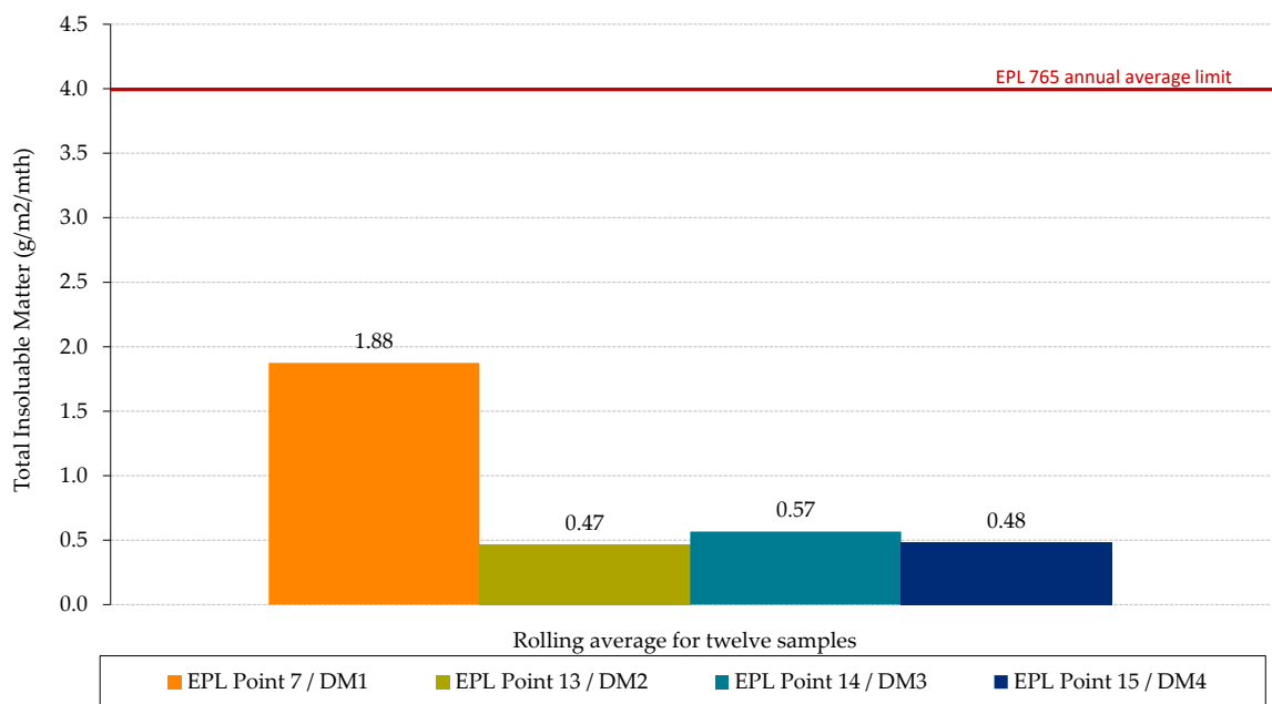
Figure 2: Rolling Average Total Insoluble Matter (12 samples until March 2022)
