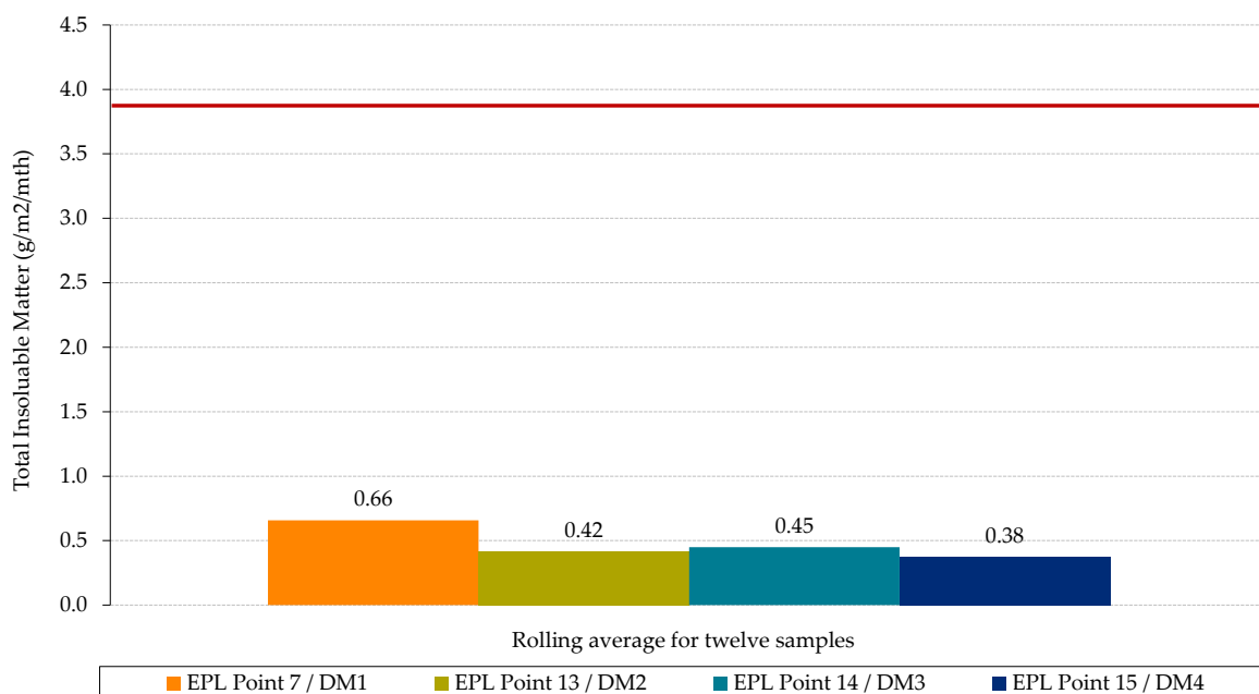
Figure 2: Rolling Average Total Insoluble Matter (12 samples until September 2021)
