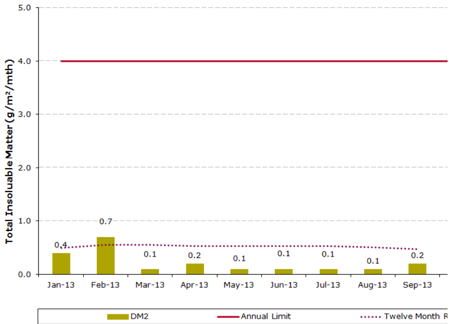
Figure 2.2: Dust monitoring gauge DM2 (EPL monitoring point No. 13)
